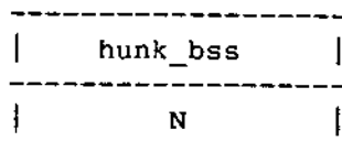
Figure 2-E: Hunk__bss (1003/3EB)
