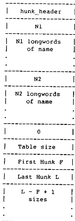
Figure 2-L: Hunk_header (1011/3F3)
