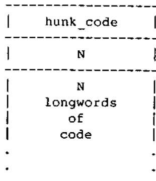
Figure 2-C: Hunk__code (1001/3E9)
