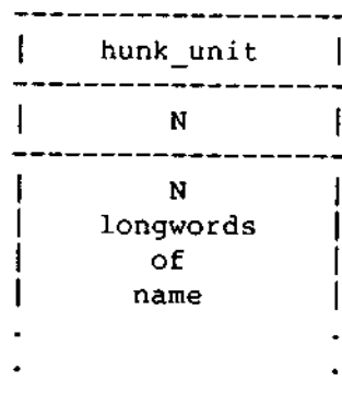
Figure 2-A: Hunk__unit (999/3E7)
