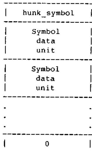
Figure 2-I: Hunk_symbol (1008/3F0)
