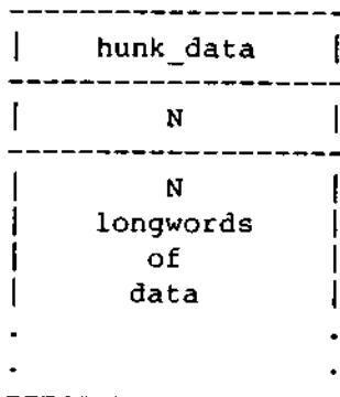
Figure 2-D: Hunk__data (1002/3EA)
