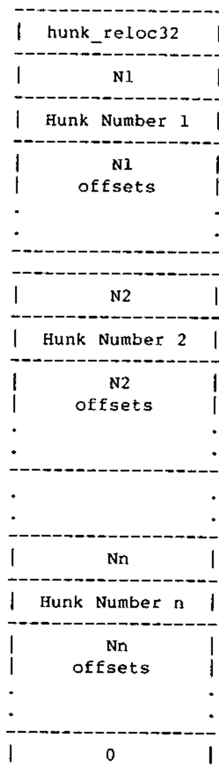
Figure 2-F: Hunk_reloc32 (1004/3EC)
