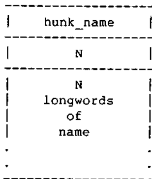
Figure 2-B: Hunk__name (1000/3E8)
