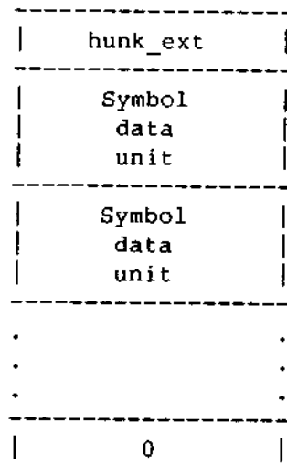
Figure 2-G: Hunk__ext (1007/3EF)
