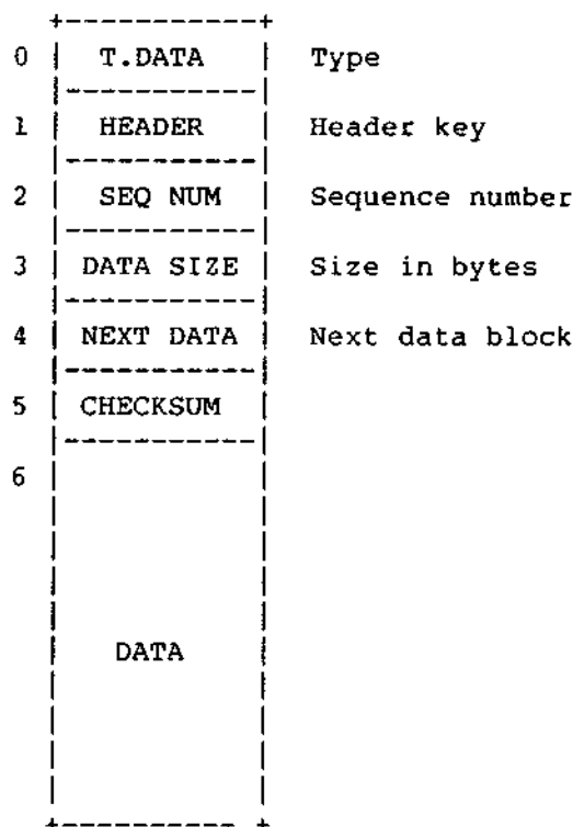
Figure 1-E: Data Block
